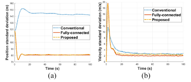
Fig. 5. Flocking control performance comparison. (a) Position standard deviation. (b) Velocity standard deviation.
