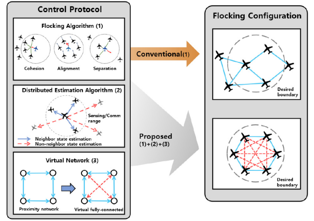
Fig. 1. Concept of an estimation-based flocking algorithm.
