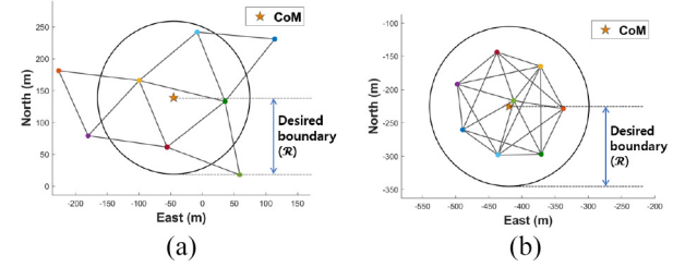
Fig. 6. Converged flock configuration. (a) Conventional flocking algorithm. (b) Proposed flocking algorithm.
