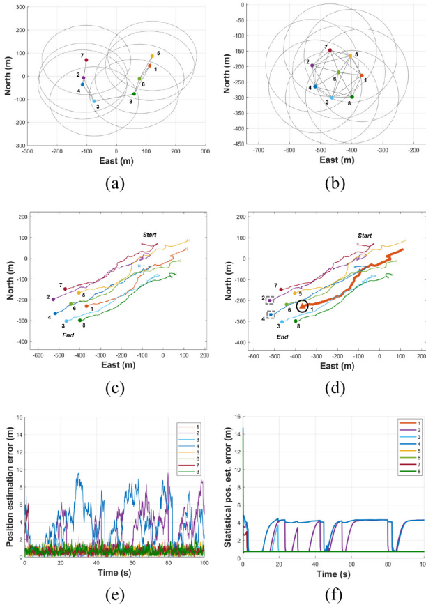
Fig. 4. Performance of flocking control with the distributed estimation under a time-varying network topology. (a) Initial network. (b) Final network. (c) True trajectory. (d) Estimated trajectory. (e) Position estimation error for each agent from the first agent's perspective. (f) Statistical position estimation error for each agent from the first agent's perspective.
