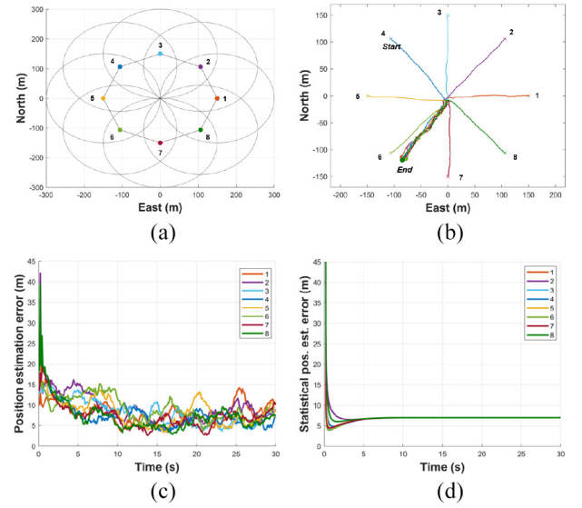
Fig. 2. Performance of rendezvous control with the distributed estimation under a fixed network topology. (a) Network. (b) Trajectory. (c) Position estimation error. (d) Statistical position estimation error.
