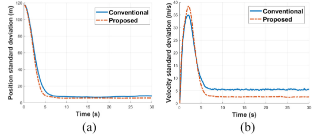
Fig. 3. Rendezvous control performance comparison. (a) Position standard deviation. (b) Velocity standard deviation.
